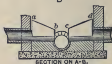
FIG. 5. JUNCTION MANHOLE.
